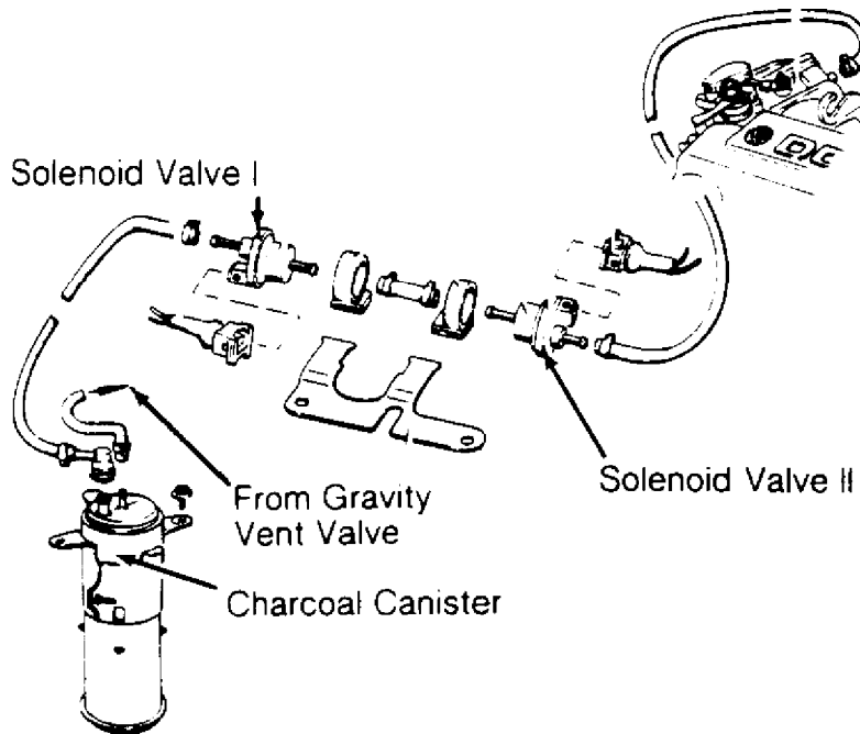
90116640 Fig. 7: Canister-to-Intake Manifold Vacuum Diagram (CIS-E Motronic System) Courtesy of Volkswagen United States, Inc.
